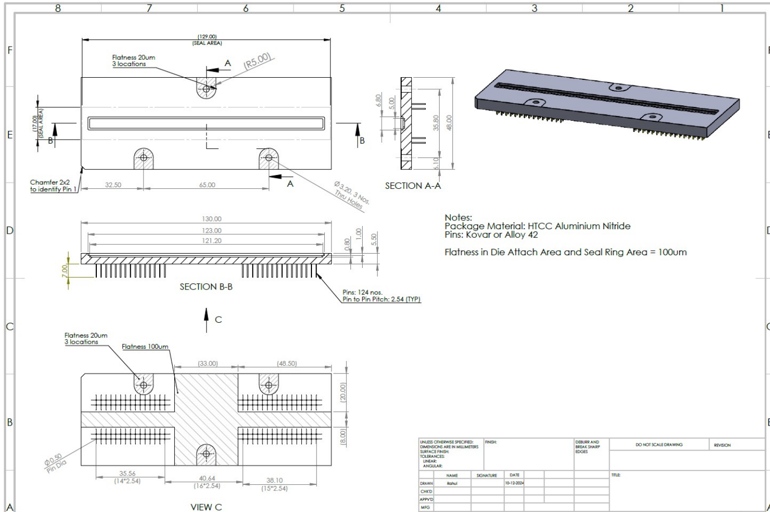
Tentative Package Drawing
